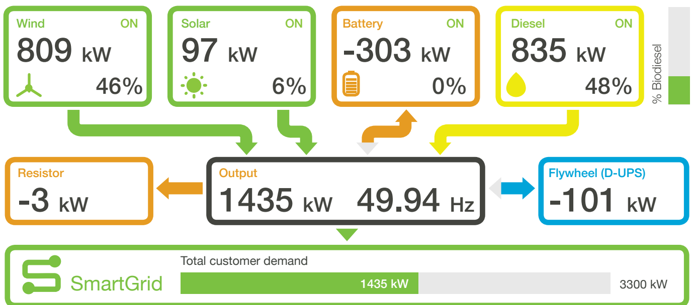
Figure 8: Snapshot of King Island’s electricity supply at 11.36am, Friday 4 September
